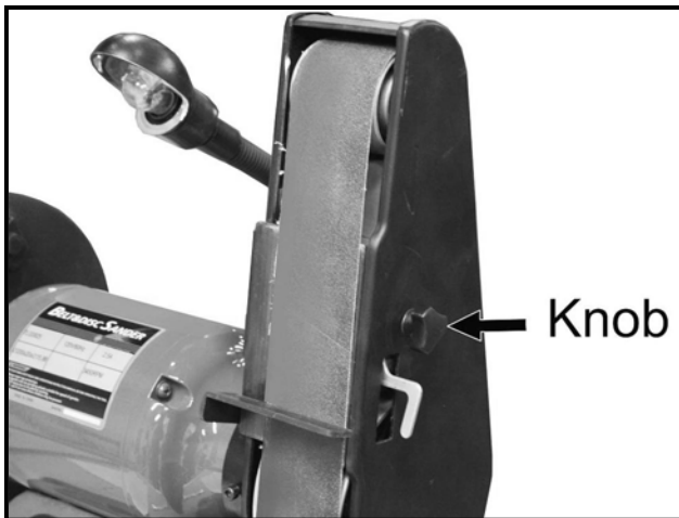
Figure-10 Removing the sanding belt cover
