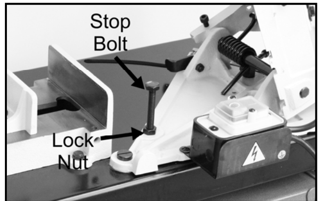
Figure-13 Stop bolt
