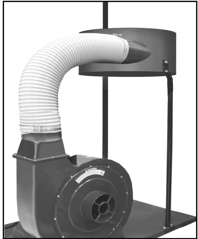
Figure-9 Connecting the hose from the outlet connector to the collector ring
