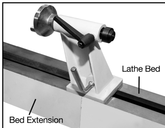
Figure-3 Sliding the tailstock onto the lathe bed and bed extension
